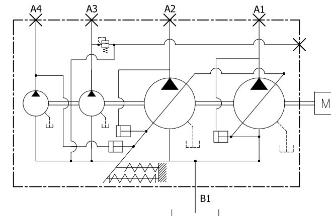
HYDRAULIC CIRCUIT FOR PRINCIPLE
