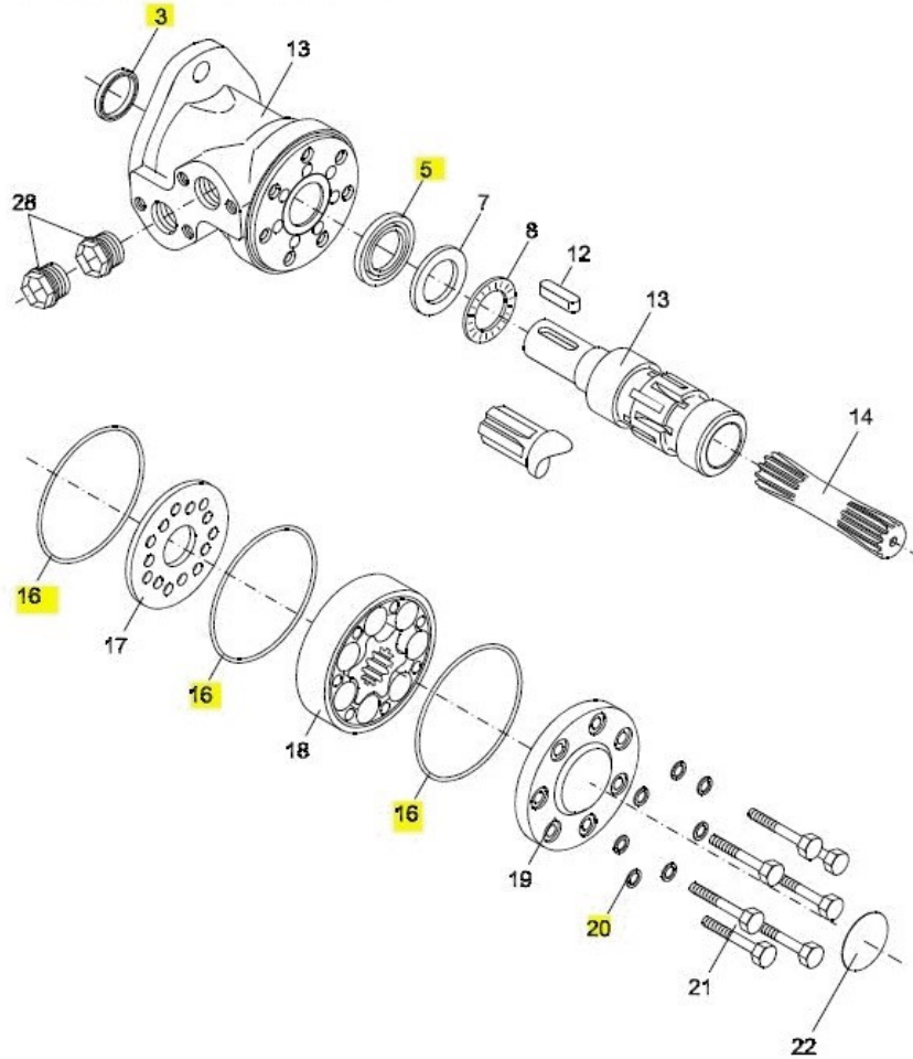
Exploded View OMR, Metric Version Series 6 with Integrated Spigot Flange
