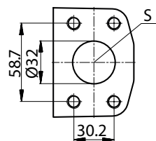
SAE 1 1/4" 3000 PSI
