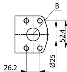
SAE 1" 3000 PSI
