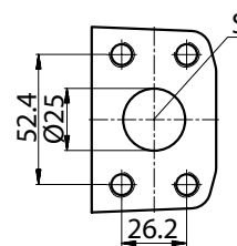
SAE 1" 3000 PSI
