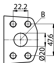
SAE 3/4" 3000 PSI
