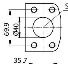
SAE 1 1/2" 3000 PSI
