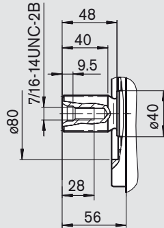
T Zahnwelle 1 1/4 in 14T 12/24DP 1) (SAE J744 – 32-4 (C))
