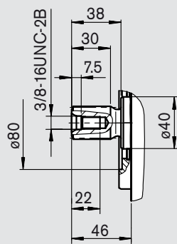
S Zahnwelle 1 in 15T 16/32DP 1) (SAE J744 – 25-4 (B-B))
