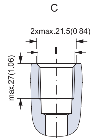
C: NPTF Hauptanschlüsse I: \frac{1}{2} - 14 NPTF
